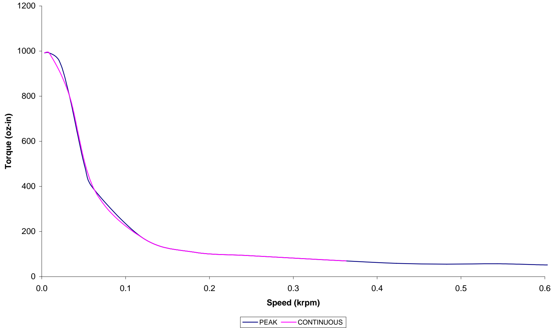
ST3430 Torque vs. Speed (24 VDC) using a PS24V8A power supply (10% Derated Torque)
