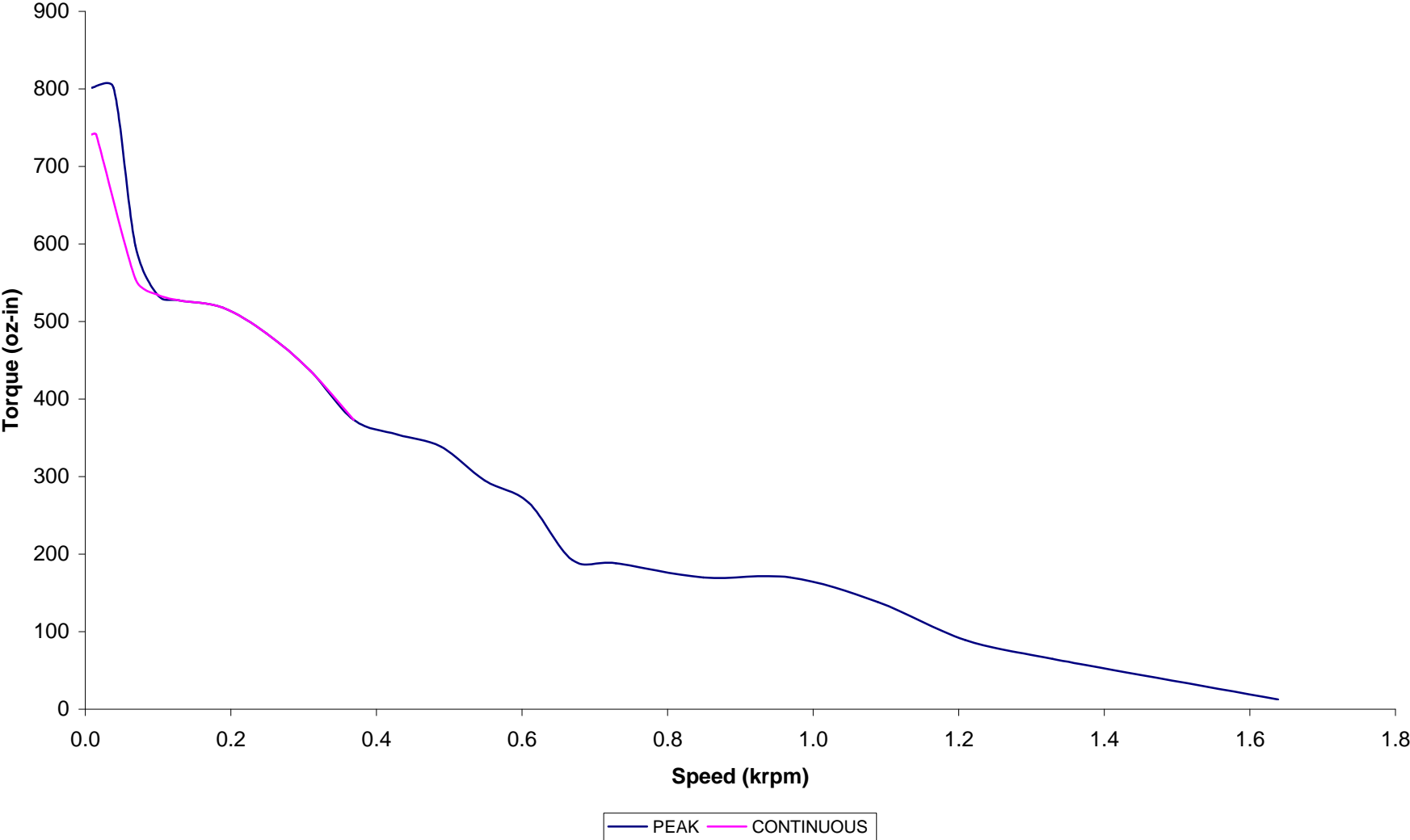
ST3420 Torque vs. Speed (75 VDC) using a PS75V6AF power supply (10% Derated Torque)
