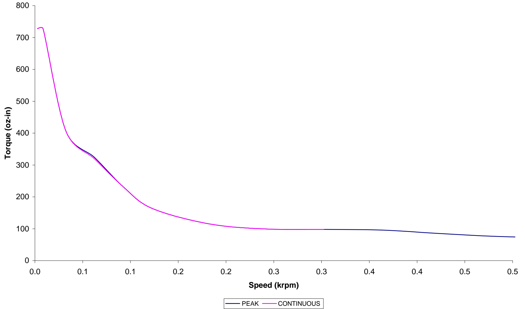
ST3420 Torque vs. Speed (24 VDC) using a PS24V8A power supply (10% Derated Torque)
