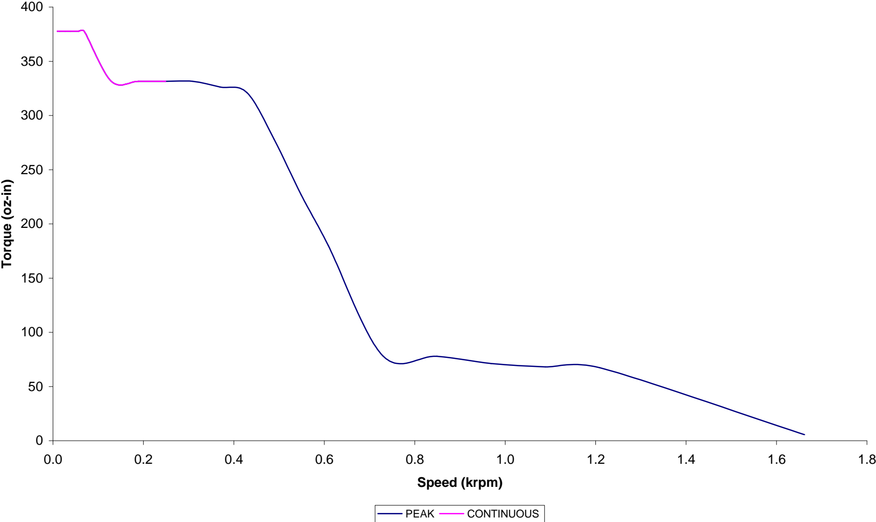
ST3410 Torque vs. Speed (75 VDC) using a PS75V6AF power supply (10% Derated Torque)
