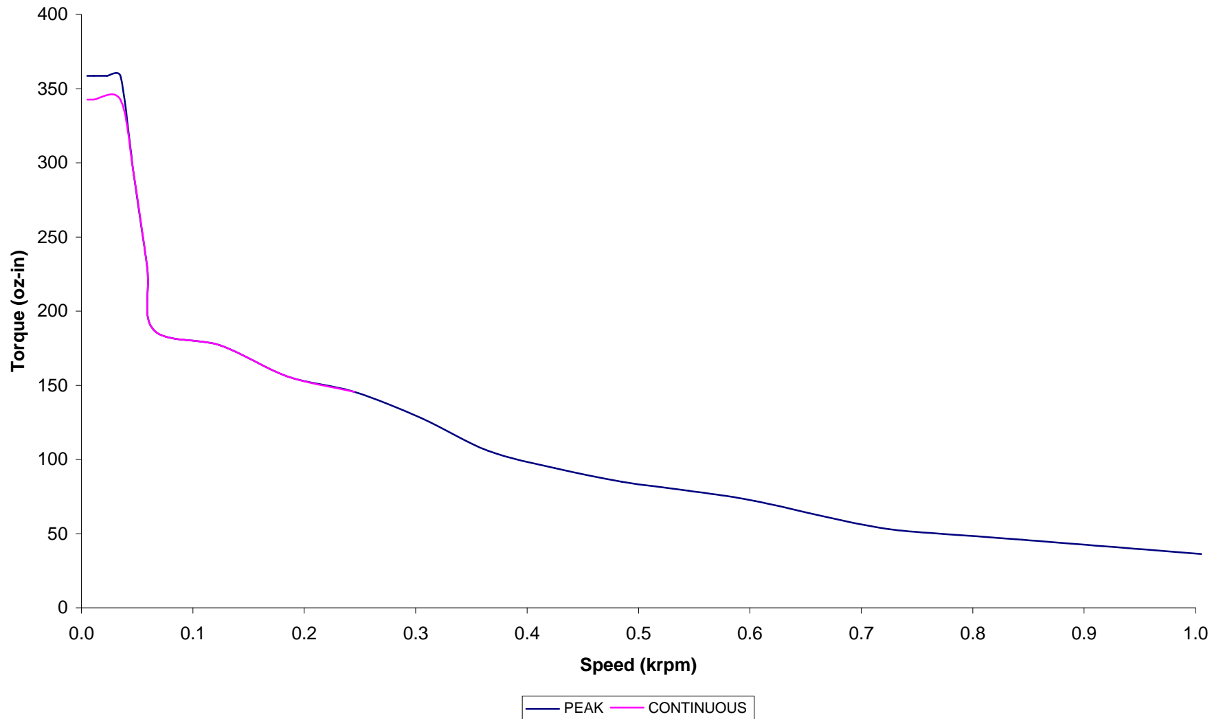
ST3410 Torque vs. Speed (24 VDC) using a PS24V8A power supply (10% Derated Torque)
