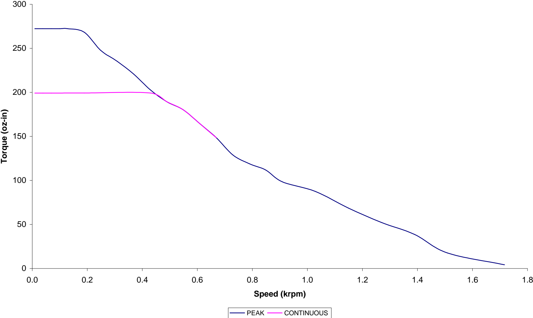
ST2330 Torque vs. Speed (75 VDC) using a PS75V6AF power supply (10% Derated Torque)
