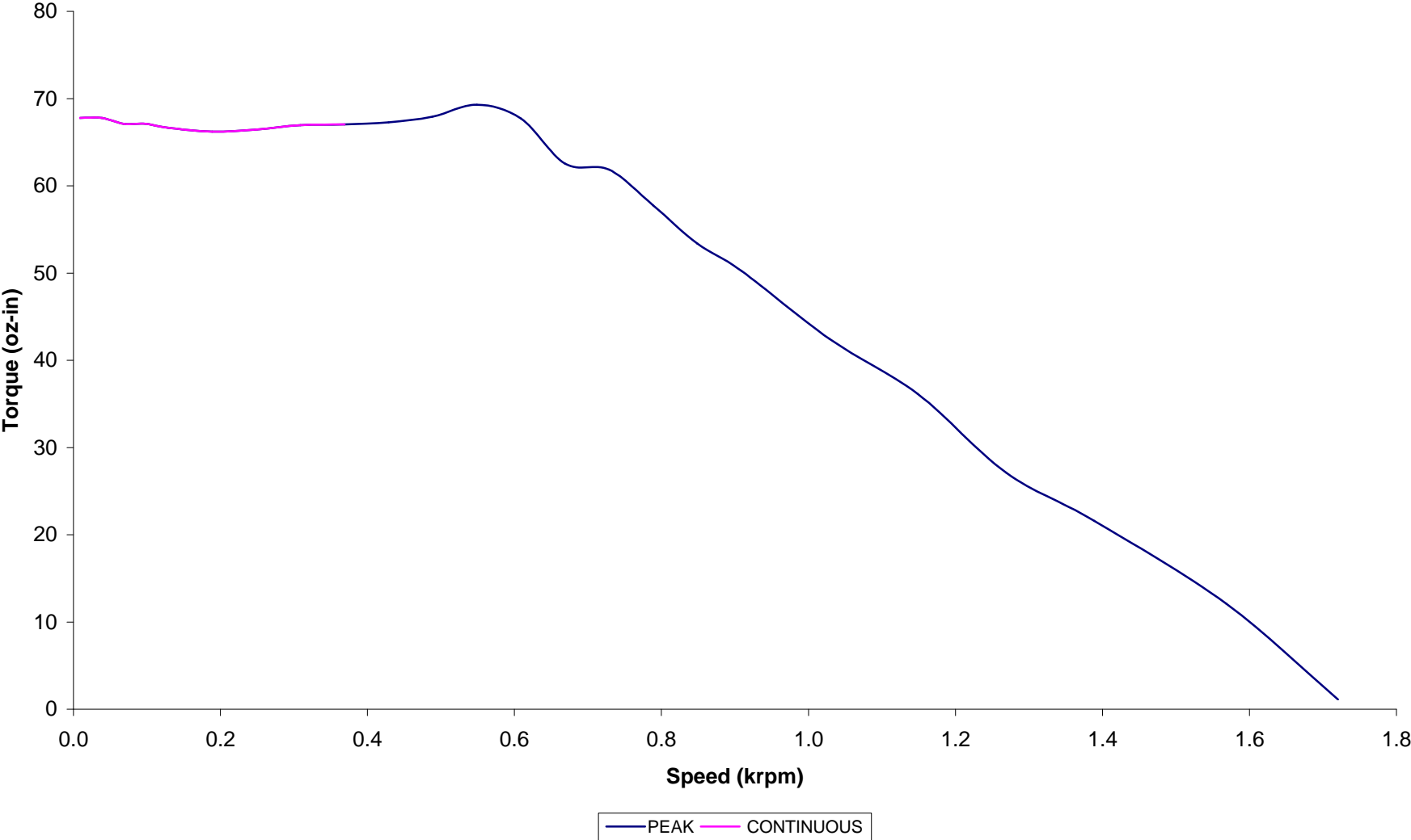
ST2310 Torque vs. Speed (75 VDC) using a PS75V6AF power supply (10% Derated Torque)
