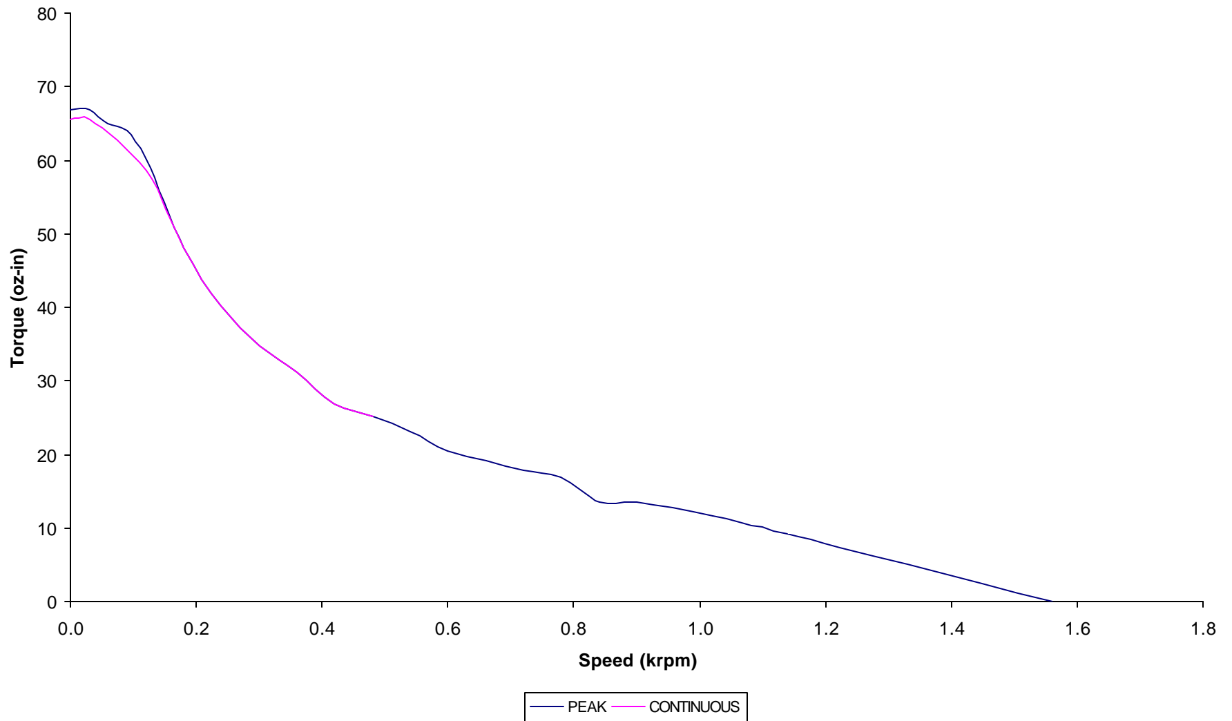
ST2310 Torque vs. Speed (24 VDC) using a PS24V8A power supply (10% Derated Torque)
