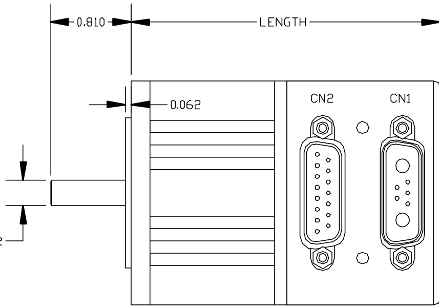
SIDE VIEW (SM2310D)
